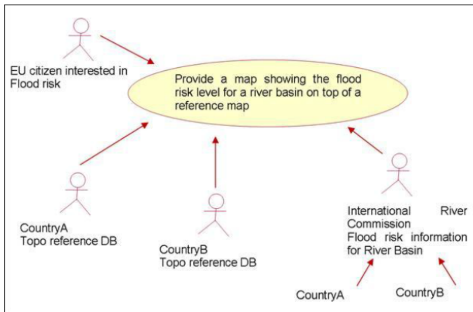
Abbildung 13: „Use case mapping“ (aus INSPIRE Data Specification on Hydrography – Technical Guidelines https://inspire.ec.europa.eu/id/document/tg/hy , Seite 150)
